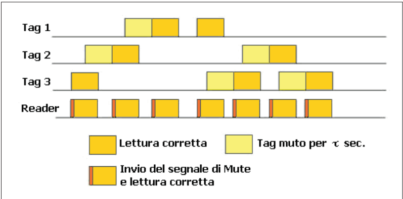
Figura A.6: Protocollo Aloha Pure Fast.
